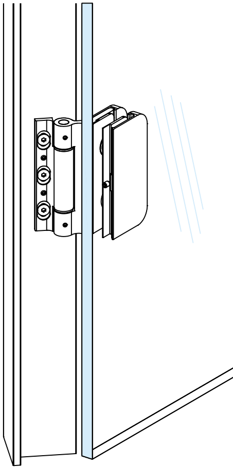
Detail Aluminium Zarge: Detail aluminium frame:
